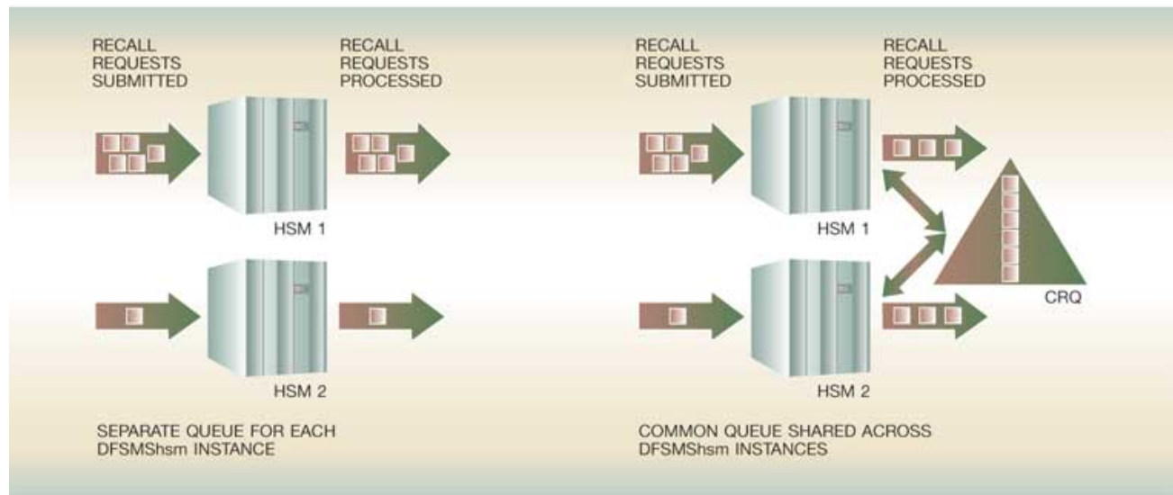
Figure 4 DFSMSHsm common recall queue
