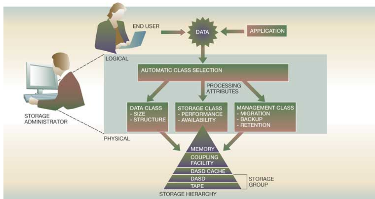
Figure 1 DFSMS policy-based storage management
