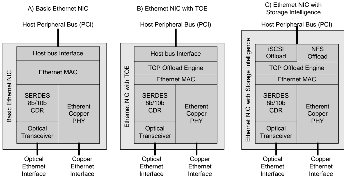
Figure 9 Ethernet NIC Functional Diagrams
